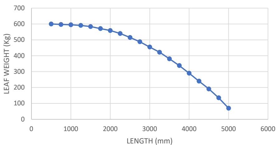
MAX LOAD / LEAF DIMENSIONS (HEIGHT 2500)
